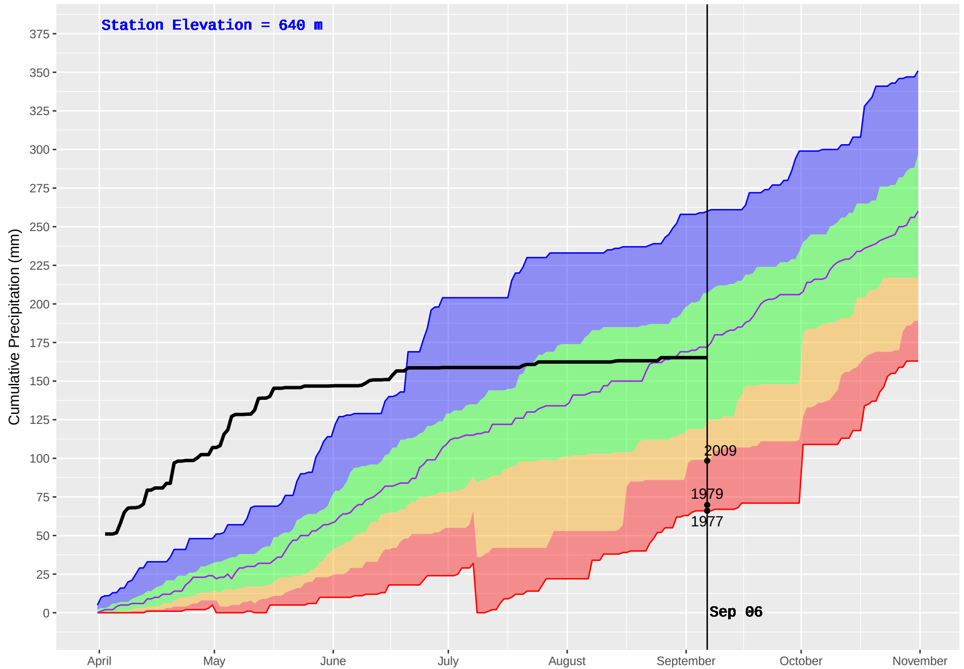
TURTLE (286) : Historical (1977–2016) and Current (2017) Noon Cumulative Precipitation
