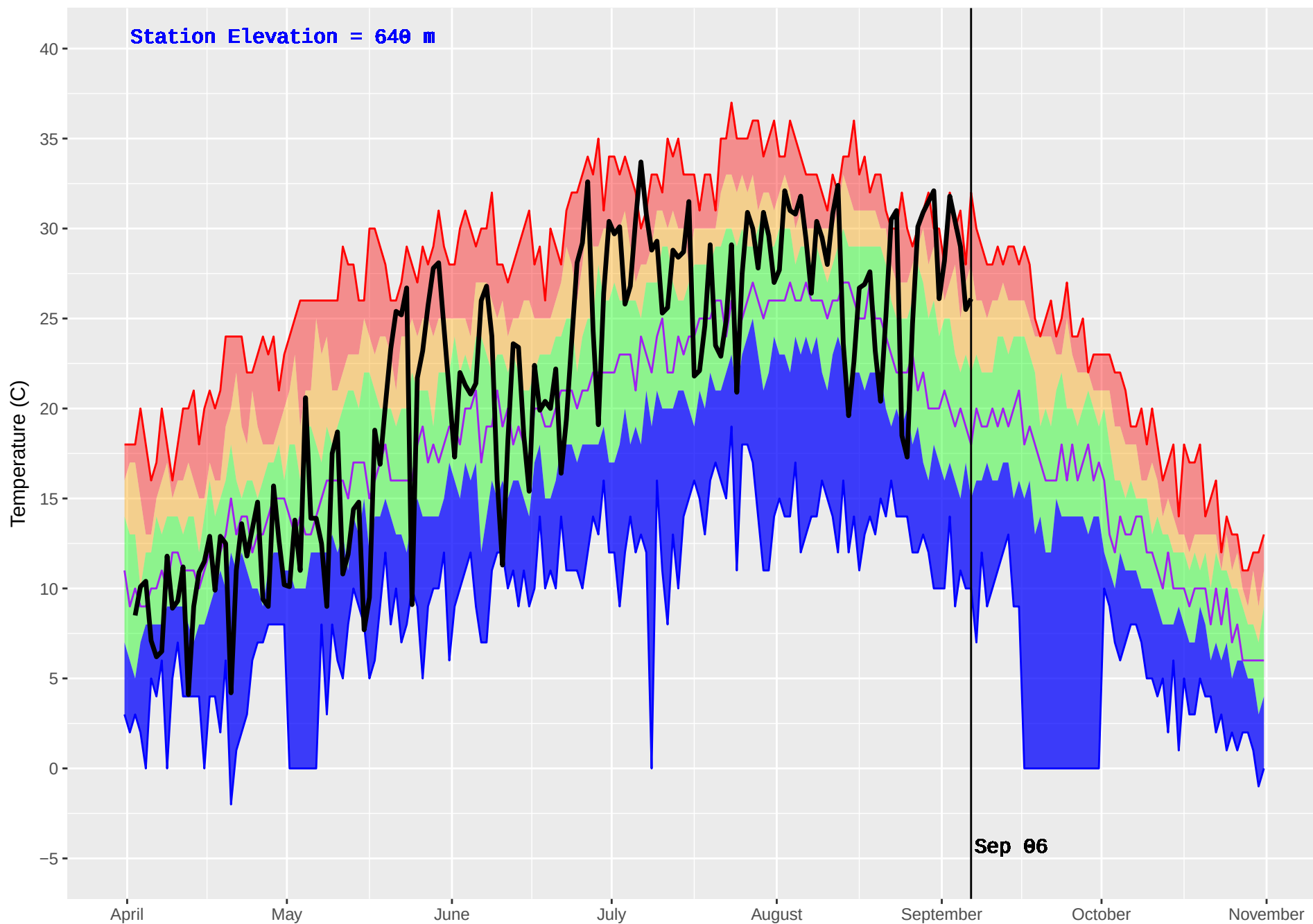
TURTLE (286) : Historical (1977–2016) and Current (2017) Noon Temperature
