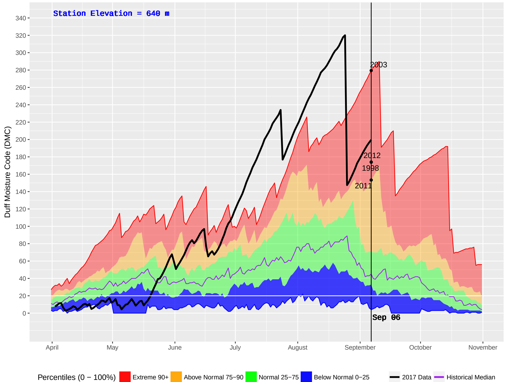
TURTLE (286) : Historical (1977–2016) and Current (2017) Noon Duff Moisture Code (DMC)
