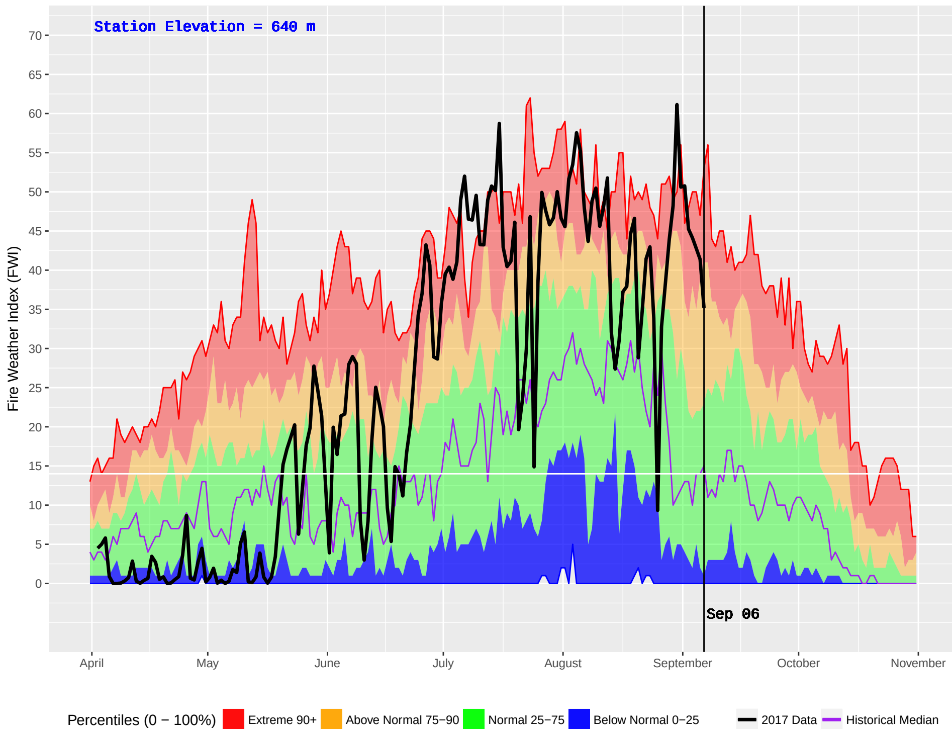
TURTLE (286) : Historical (1977–2016) and Current (2017) Noon Fire Weather Index (FWI)
