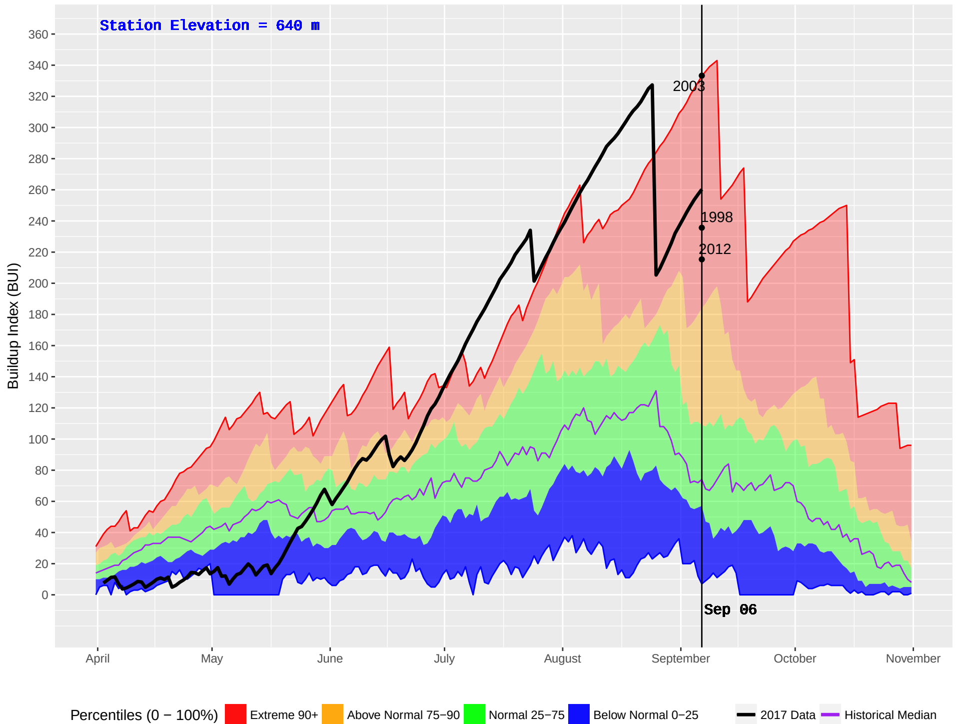
TURTLE (286) : Historical (1977–2016) and Current (2017) Noon Buildup Index (BUI)
