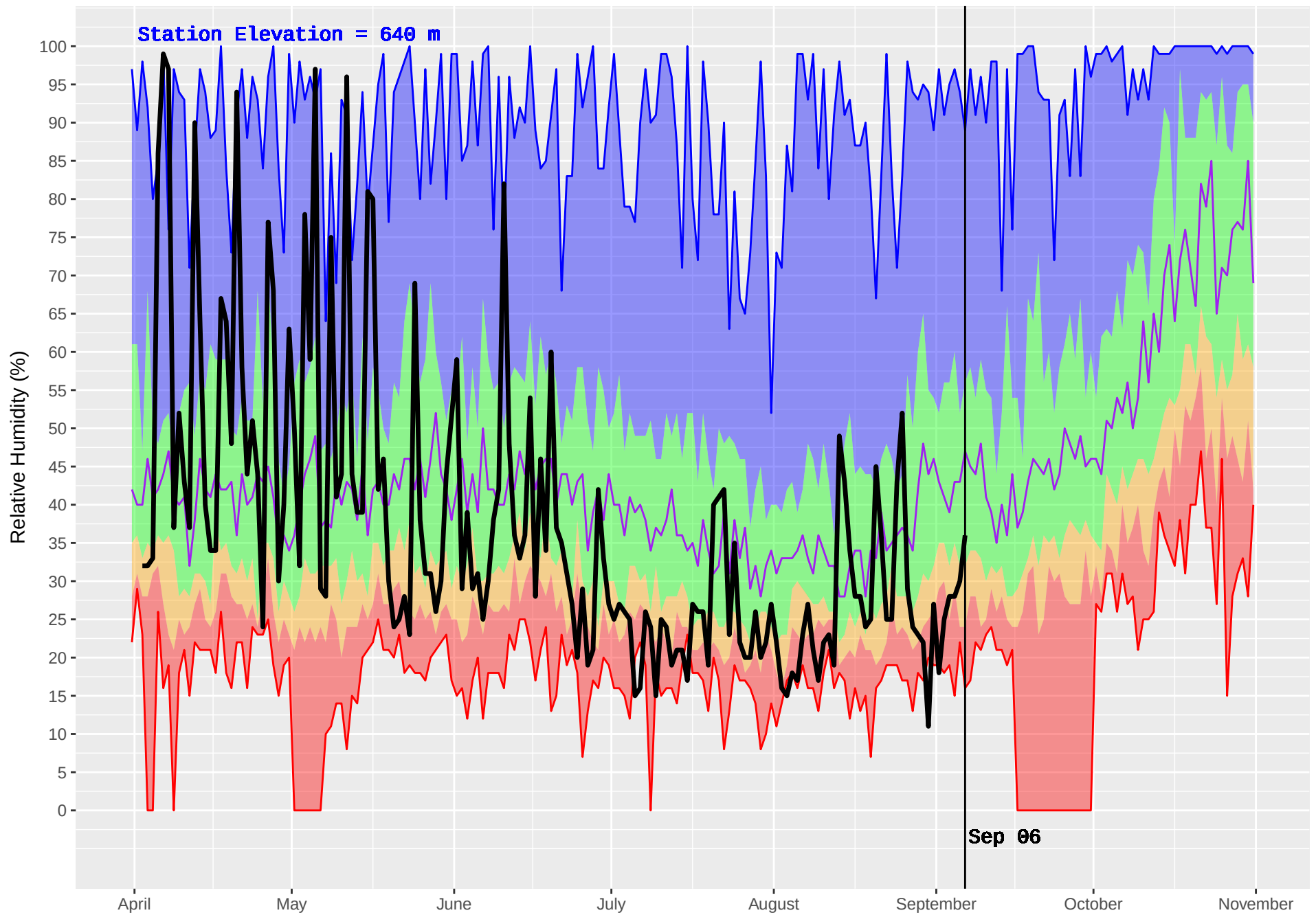
TURTLE (286) : Historical (1977–2016) and Current (2017) Noon Relative Humidity
