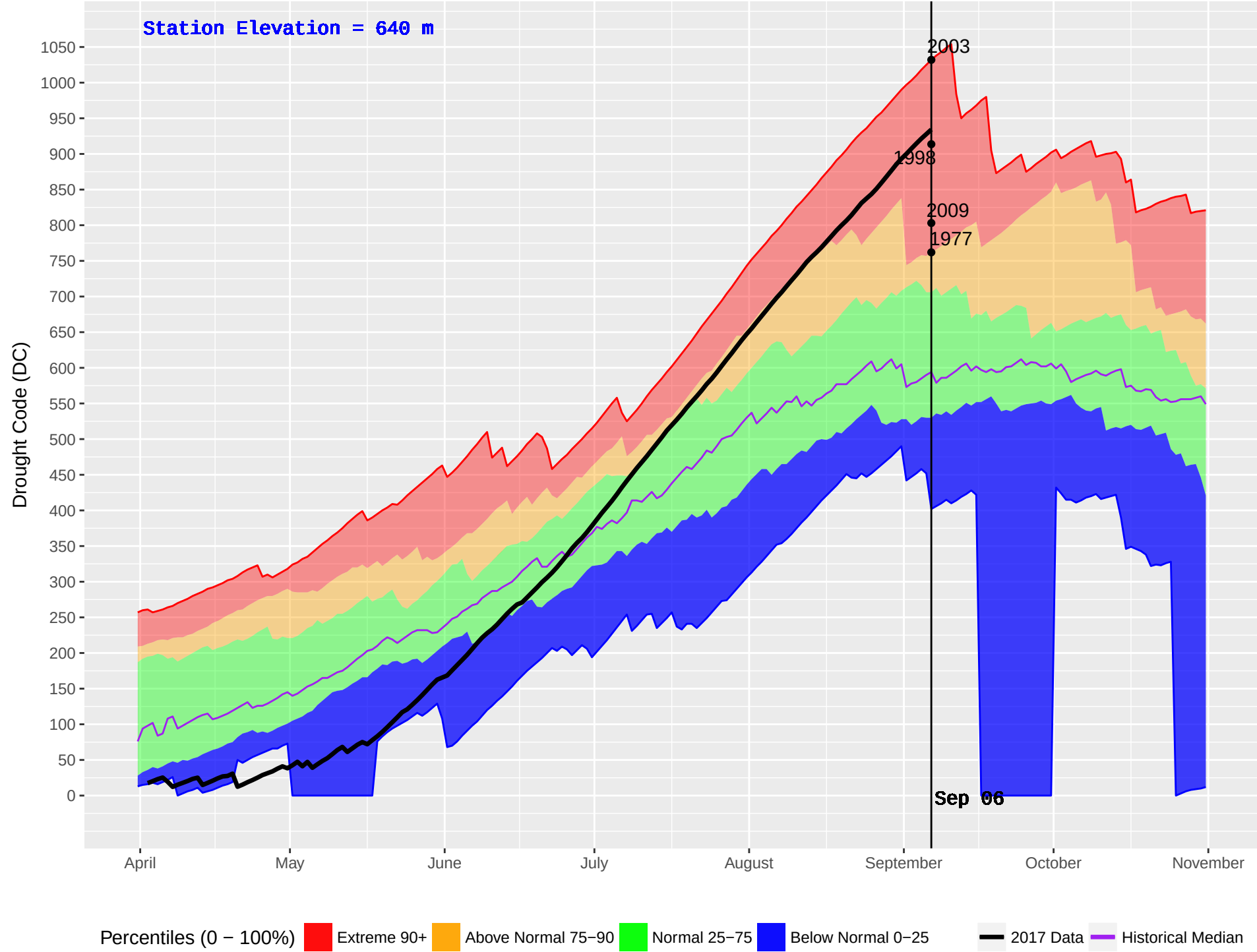
TURTLE (286) : Historical (1977–2016) and Current (2017) Noon Drought Code (DC)
